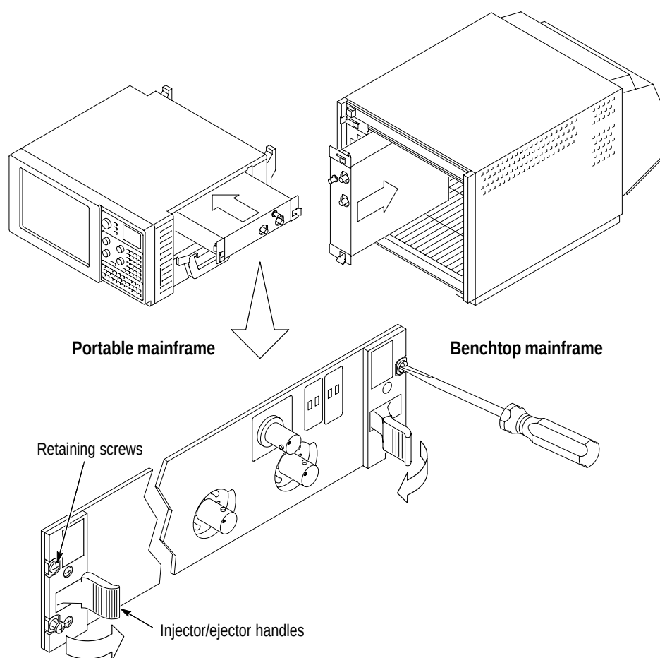
Figure 2: Installing modules
