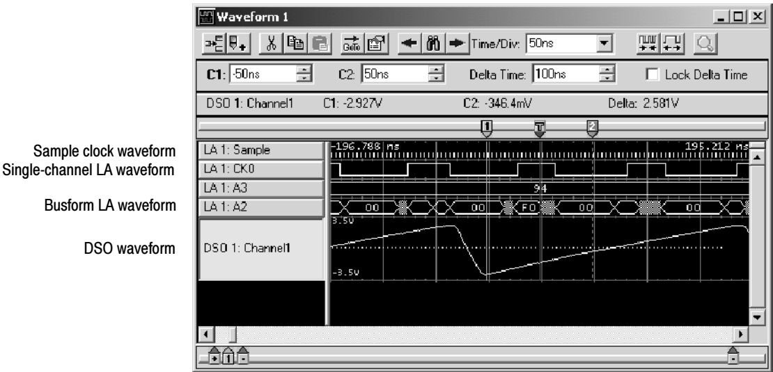
Figure 3-62: Waveform types
