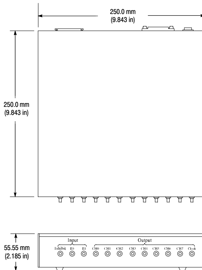
Figure 13: P6475 Variable probe dimensions
