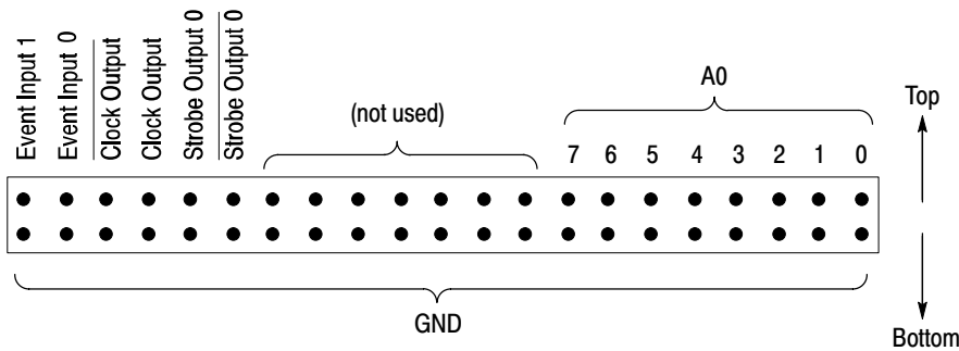
Figure 5: P6472 output connector pin assignments
