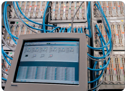
▶ Example of TLA721 with ten TLA7XM Mainframes.
