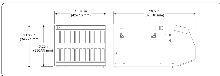
► TLA721 and TLA7XM Benchtop and Expansion Mainframes.
