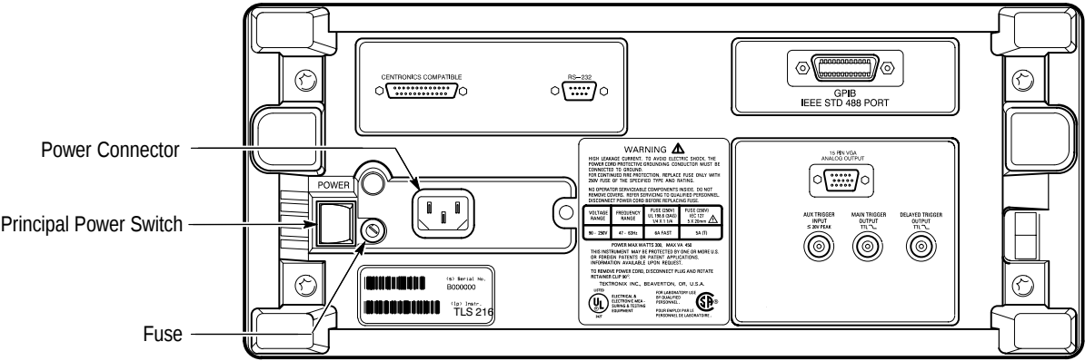
Figure 1-1: Rear Panel Controls Used in Start Up
