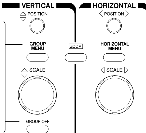
Figure 1-10: The VERTICAL and HORIZONTAL Controls
