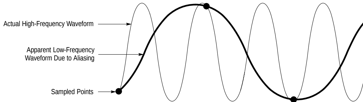
Figure 2-7: Aliasing
