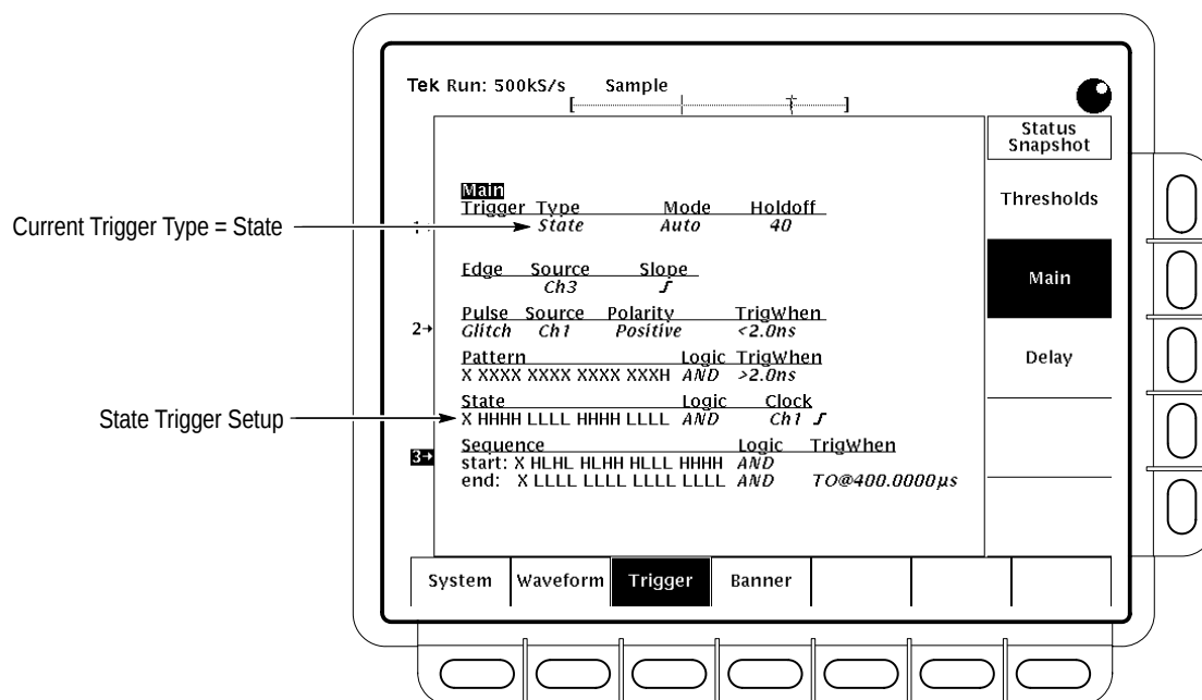
Figure 3-74: Snapshot of Trigger Status
