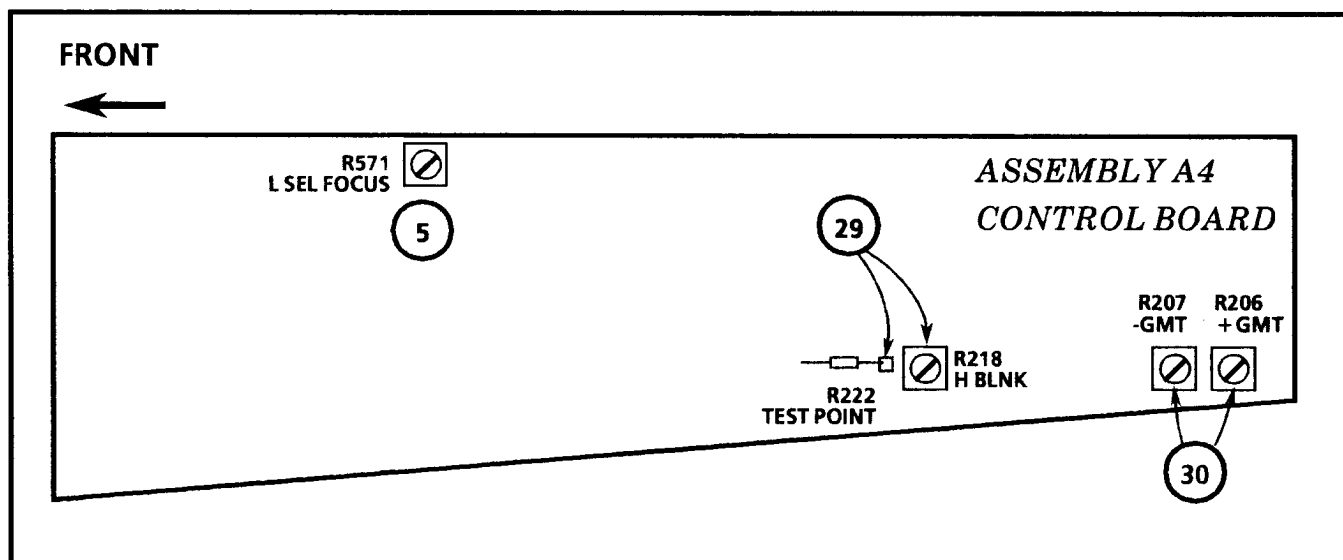
Fig. 5-17. CONTROL board, showing adjustment, jumper, and test point locations. Adjustment Procedure step numbers are shown in circles.
