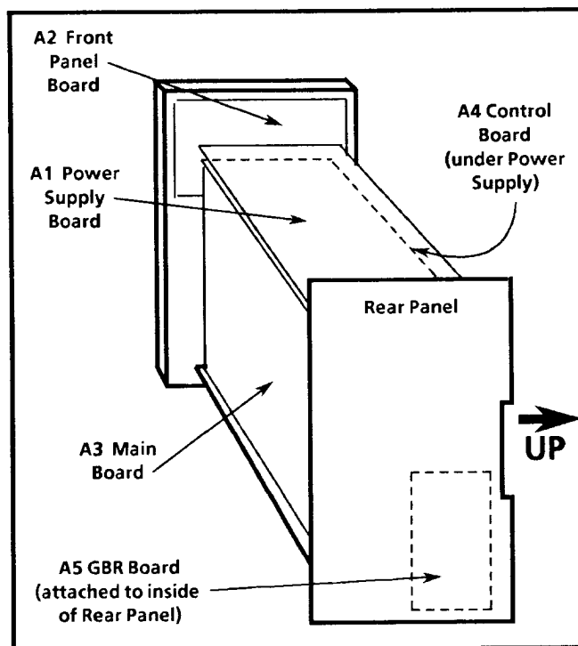
Fig. 6-2. Circuit board assembly locations.
