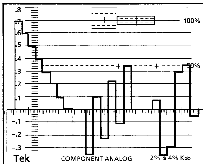
Fig. 2-10. Parade display.
