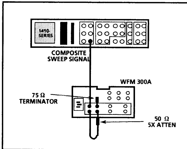
Fig. 5-18. Equipment setup for adjusting X5 high frequency compensation.
