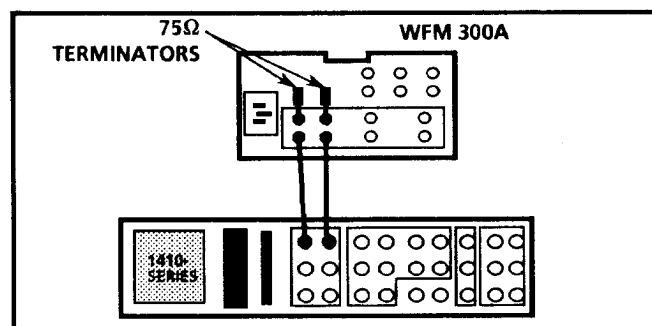
Fig. 5-6. Equipment setup for checking horizontal sweep operation.
