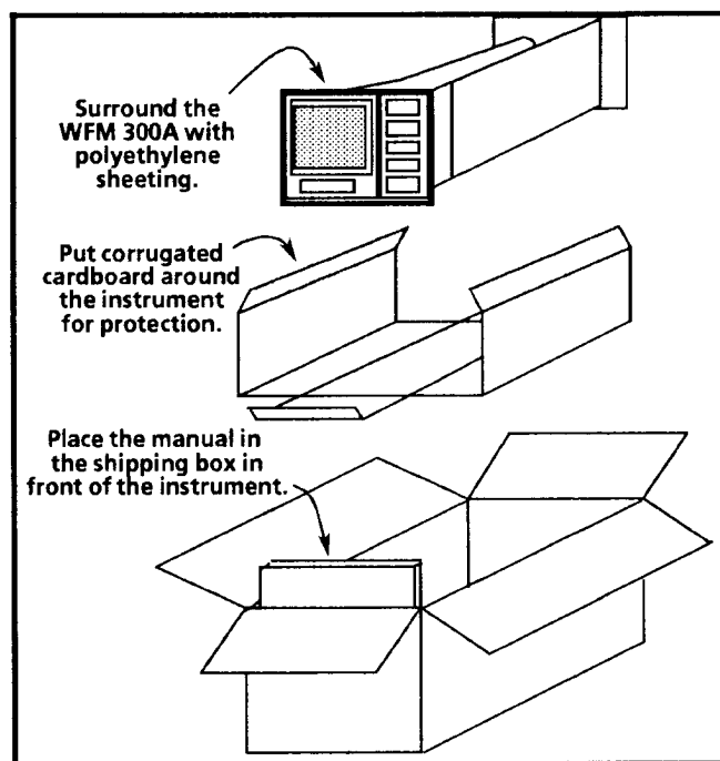
Fig. 6-9. Repackaging.
