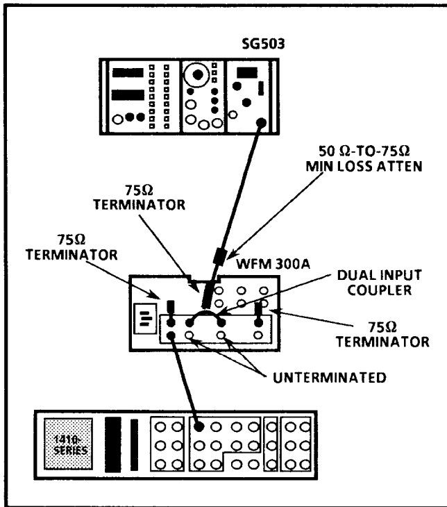
Fig. 5-8. Setup for checking Bowtie mode common mode rejection.
