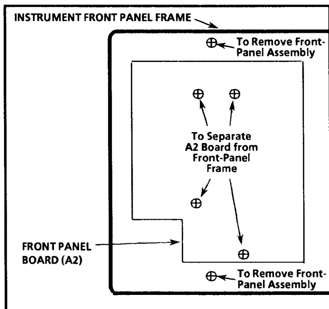
Fig. 6-6. Front Panel board (A2) securing screws.
