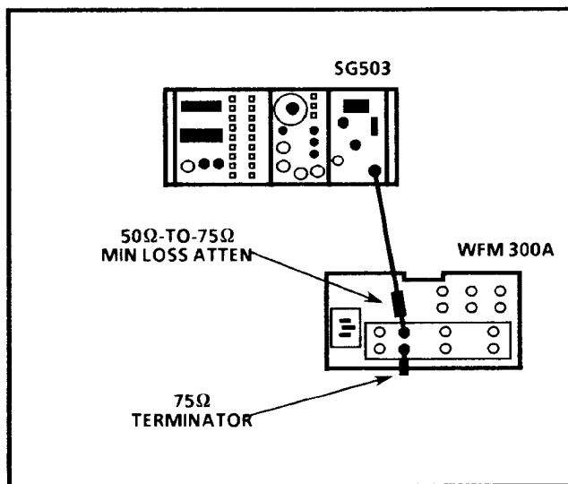
Fig. 5-4. Setup for checking frequency response .
