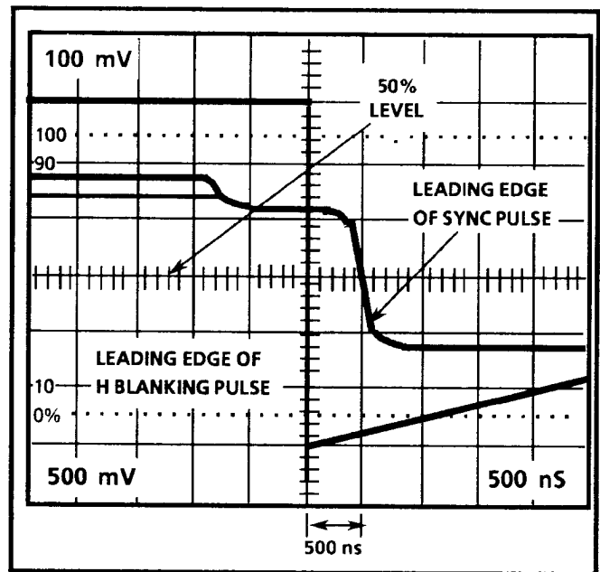
Fig. 5-23. Correct horizontal blanking pulse timing for 525/60 TV standard. Timing for 625/50 TV standard is 1 \mu s.
