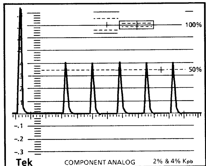
Fig. 2-11. 1 Line Sweep Mode with X5 Gain Off.
