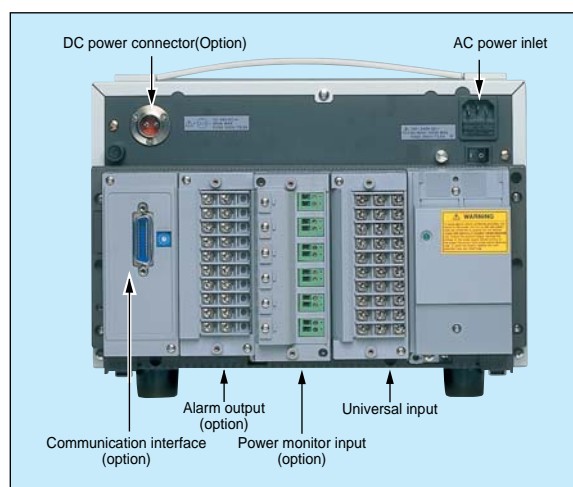
Rear view of the DR130
