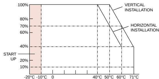
FIGURE 1 Output Power vs. Ambient Temperature
