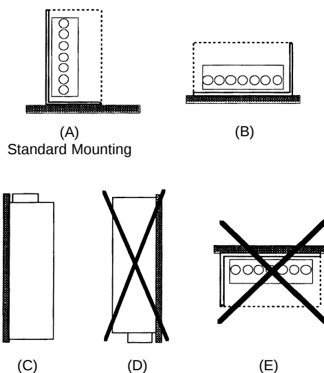
FIGURE 2 Mounting Directions 30, 50, 100, 150W Models
