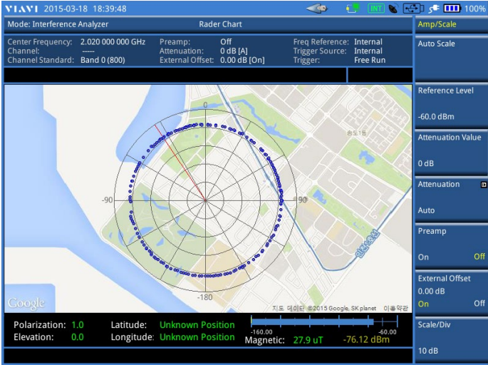
Interference analysis test — Radar Chart (measurement)
