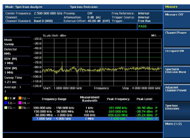
RF Test — Spurious Emissions
