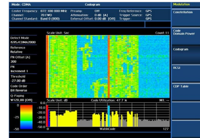
Modulation analysis — Codogram
