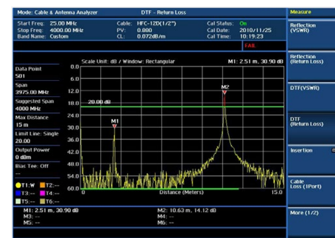
Cable and antenna test — Distance to Fault
