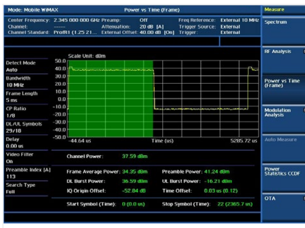
Modulation analysis — Power vs. Time
