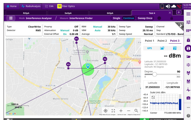
OneAdvisor Interference Finder
