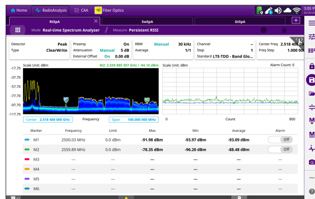
OneAdvisor RSSI Measurement
