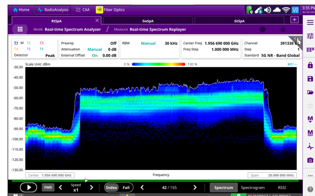
OneAdvisor Spectrum Logging and Replaying
