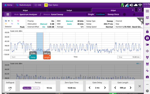
Gated Sweep Spectrum – Gate Time Setting
