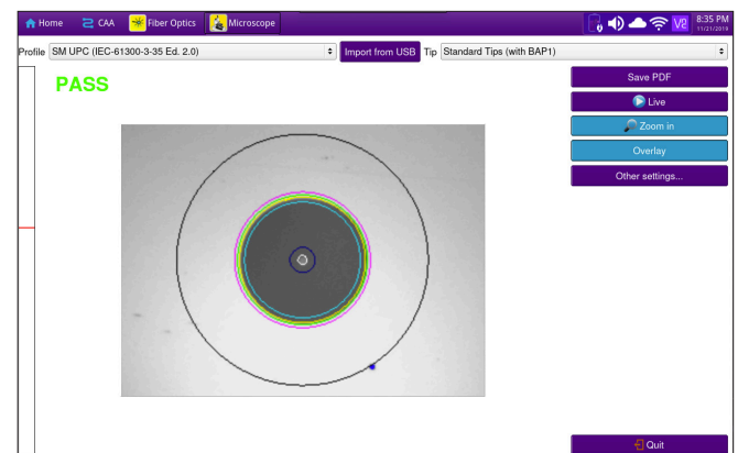
Fiber Inspection
