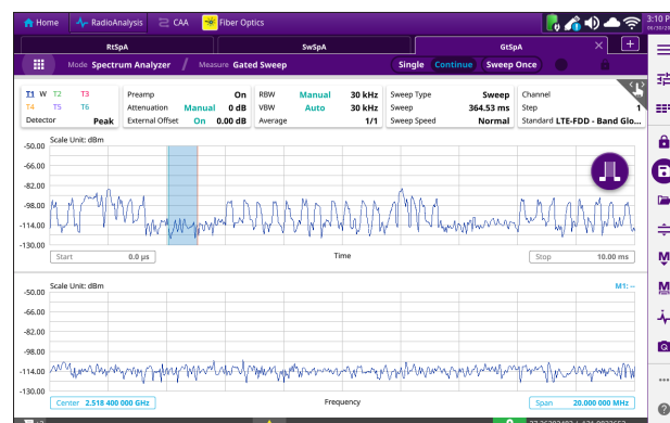
Gated Sweep Spectrum – Spectrum Analysis
